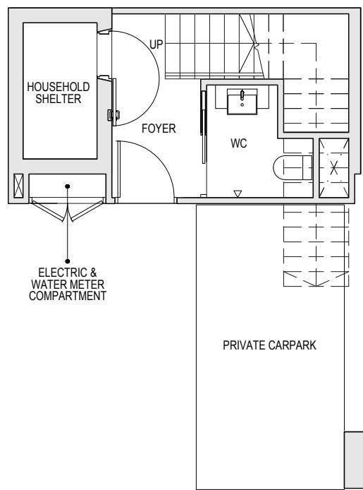
BASEMENT PLAN
