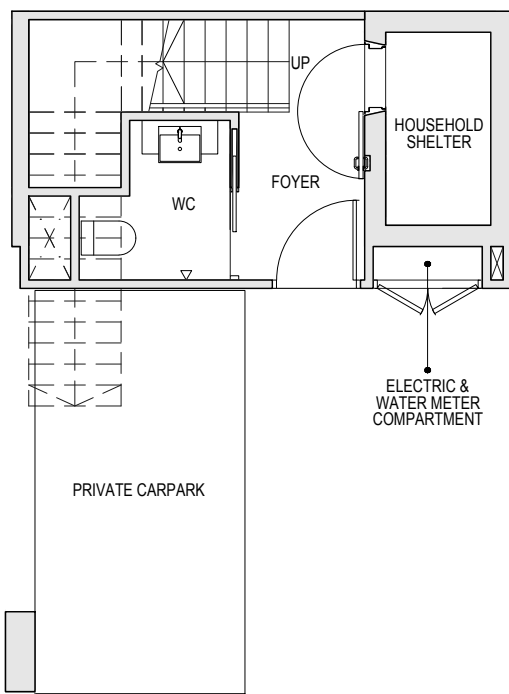
BASEMENT PLAN
