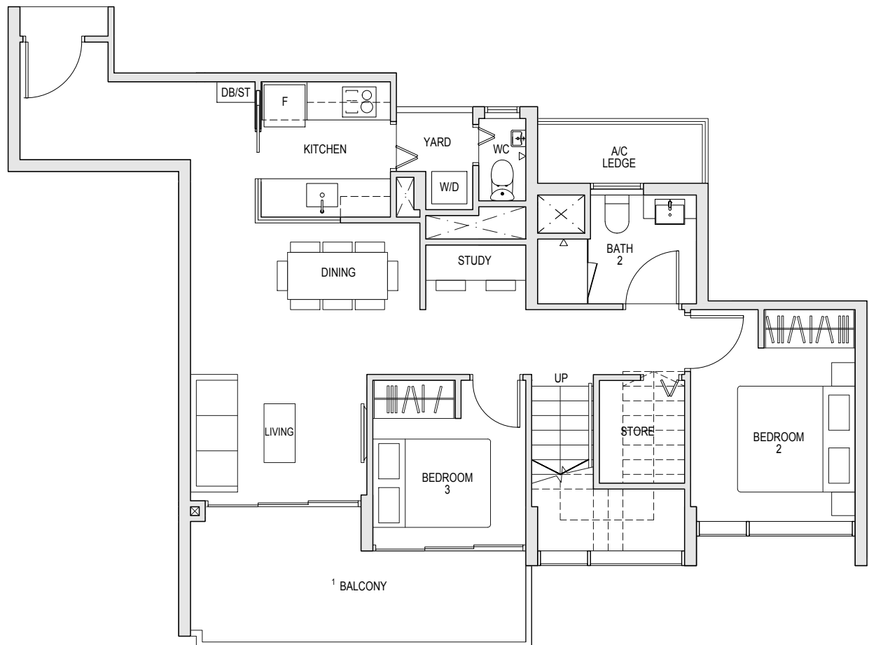
LOWER STOREY PLAN
